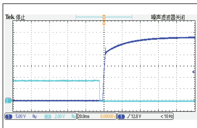
图 6: ON/OFF 启机延时, Vin=280V, Io=17.9A, TC=25°C CH1: 输出电压, CH2: ON/OFF 电压
